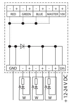
Monochrome LED strips control
