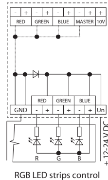
RGB LED strips control
